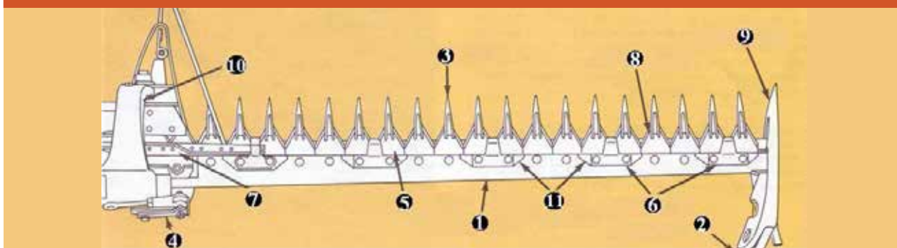
Cutter bar (1-Bar 2- Grass board 3- Guard 4- Inner shoe 5- Knife assembly 6- Knife clips 7- Knife head 8- Knife section 9- Outer shoe 10- Yoke 11- Wear plate)
