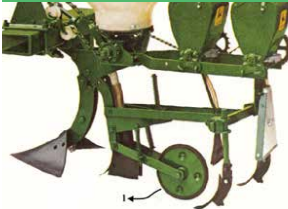
1-Seed packer wheel
