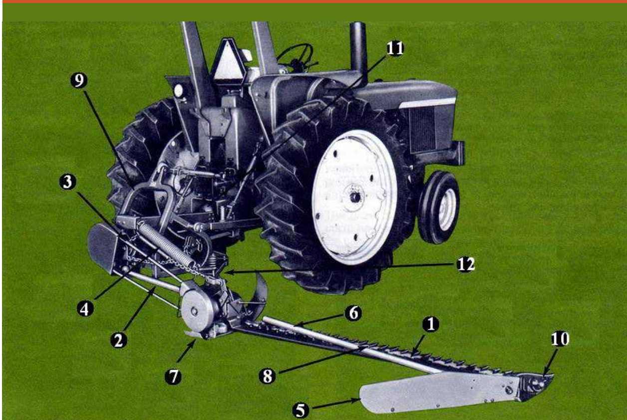
Cutter bar mower
