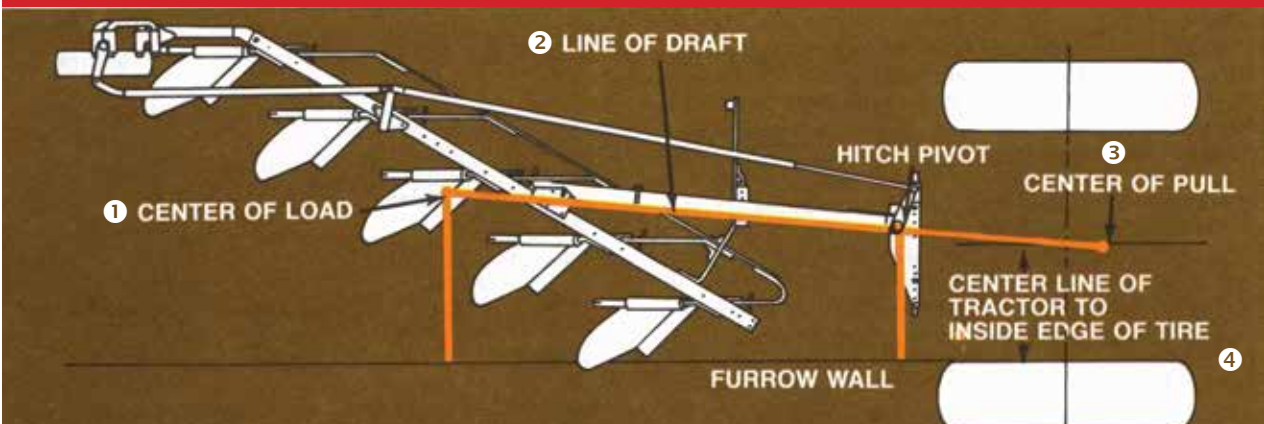
1- Center of Load 2- Line of draft 3- Center of pull 4- Tractor center line
