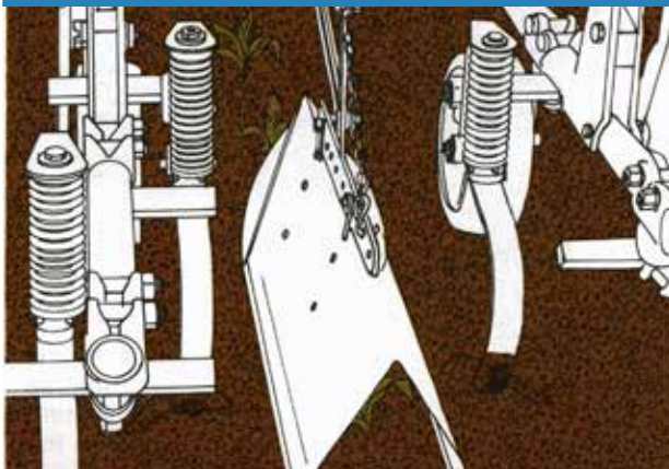
Hooded cultivator = Cultivator with crop shields
